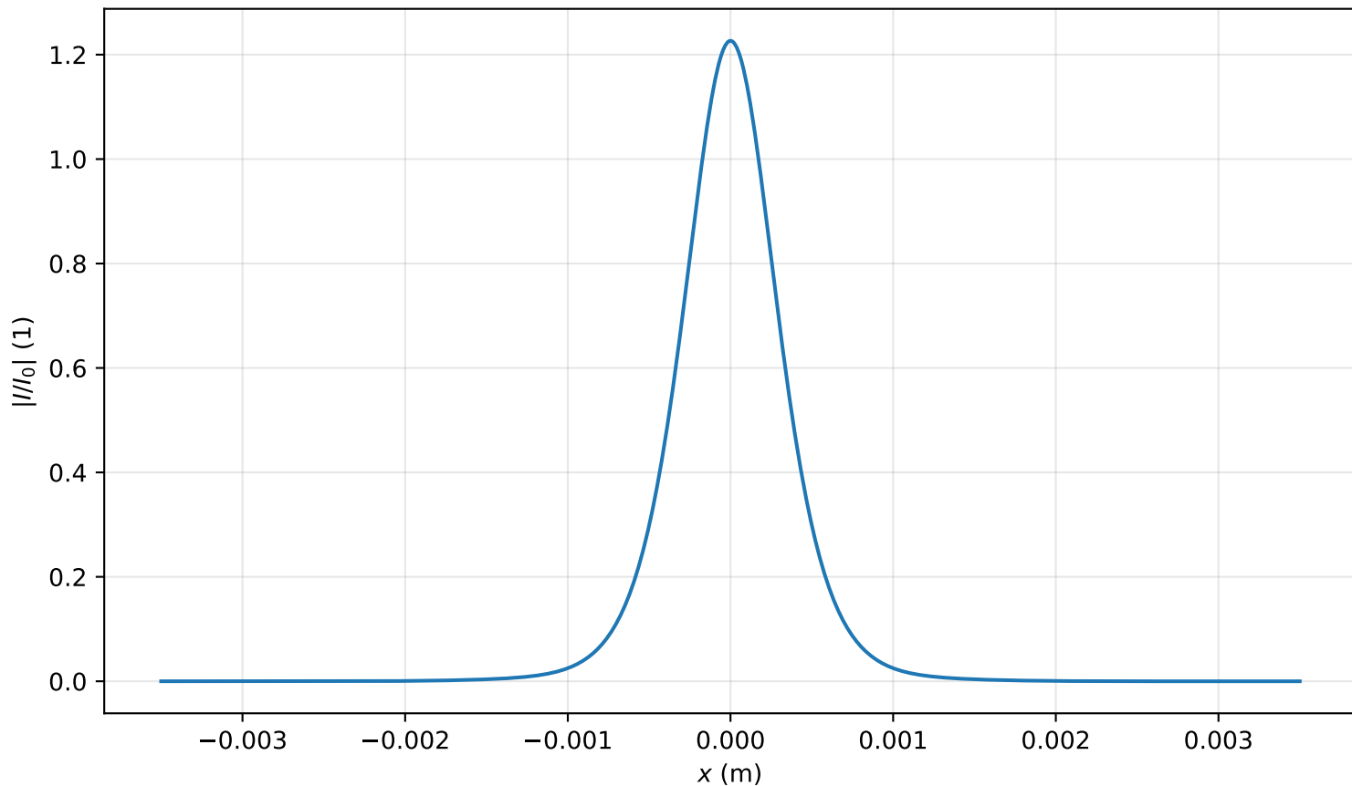
Intensity profile I(x, y = 0, z = 2.468m)/I_0 , P_{in}=0.8P_{cr} , artificial time
